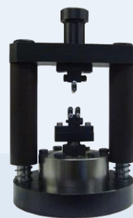
3 points microflexure fixture with load cell.
