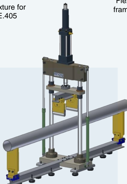
ME-406 testing frame design with 4 points flexure fixtures. Roller distance between 400 and 2500 mm.
