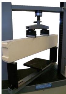
Insulators, flexure strength EN 12089
